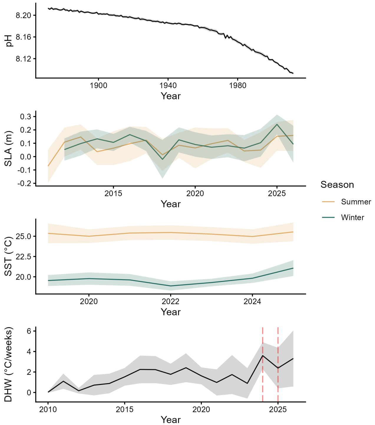
Figure B.1: Seasonal sea level anomaly, seasonal sea surface temperature and Degree Heating Weeks at the scale of the HMP. Solid lines represent mean values for sea level anomaly (SLA), sea surface temperature (SST) and Degree Heating Weeks (DHW). Confidence bounds represent standard errors. Red dashed vertical lines represent maximum DHW values that are plotted spatially in Figure 4.
