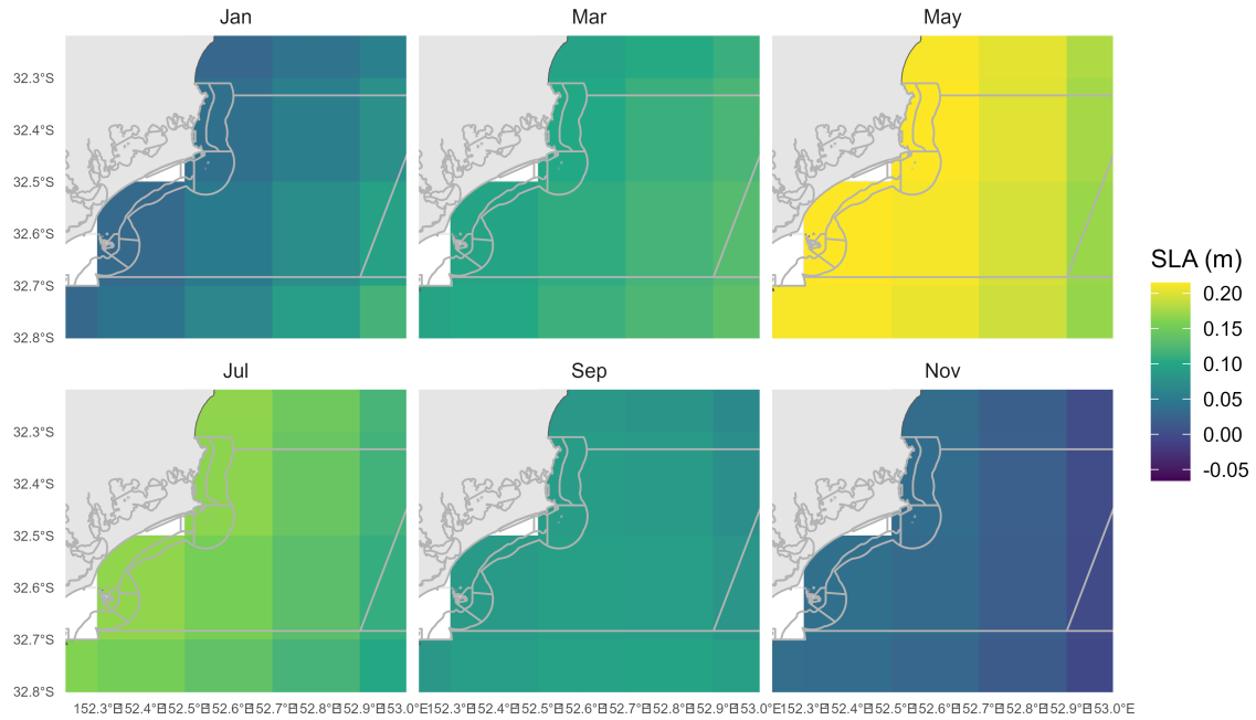
Figure B.2: Sea level anomaly, as an index of upwelling, at the scale of the HMP. Heatmap values represent high (yellow) and low (blue) bimonthly sea level anomaly (SLA). Grey polygons represent State spatial management and Australian Marine Park boundaries.
