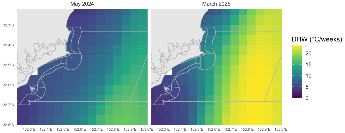
Figure B.4: Maximum Degree Heating Weeks at the scale of the Hunter Marine Park. Heatmap values representing high (yellow) and low (blue) monthly Degree Heating Weeks (DHW) for the two most recent marine heatwave periods on record. Grey polygons represent State spatial management and Australian Marine Park boundaries.
